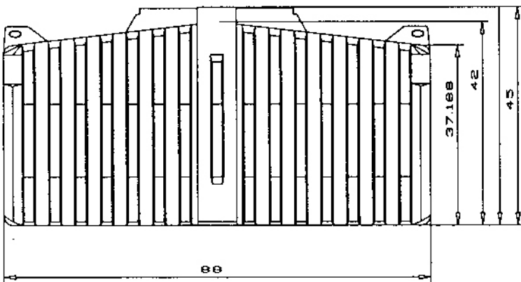
PART # 40969 END VIEW
