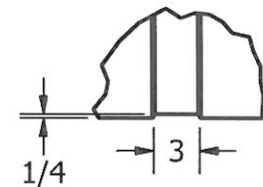
DETAIL A SCALE 1 / 12
